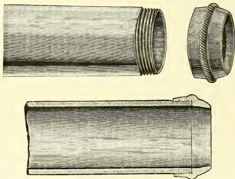
Roper's Detachable Choke-muzzle.
